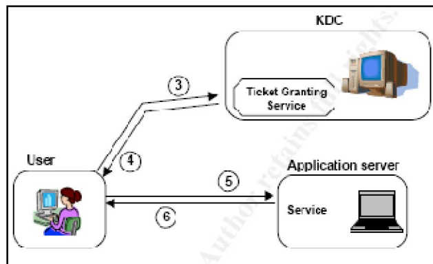
Gambar 2. Ticket Granting Service
