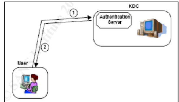
Gambar 1. Authentication Service
